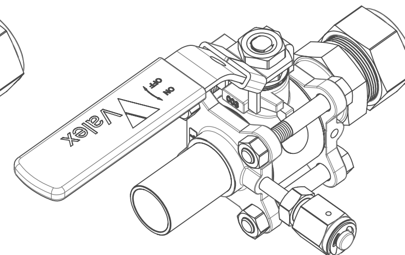
STANDARD FINISH OPTION SHOWN WITH OPTIONAL FACE-SEAL PURGE PORT (COMPRESSION PURGE ALSO AVAILABLE)
