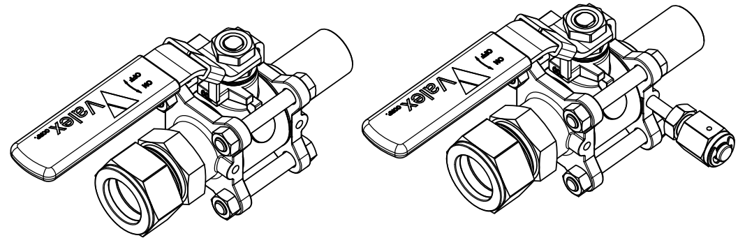
STANDARD FINISH OPTION SHOWN WITH OPTIONAL FACE-SEAL PURGE PORT (COMPRESSION PURGE ALSO AVAILABLE)
